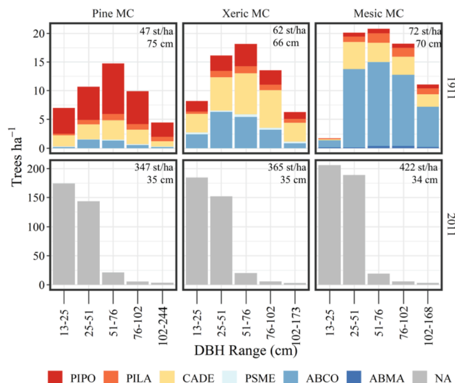
Fig. 2. For pine-mixed conifer, xeric-mixed conifer, and mesic-mixed conifer forest types the diameter distribution of the 1911 historical (top panels) and 2011 contemporary (bottom panels) datasets by DBH size classes (indicated by the range in DBH values) and species (1911 only). Density (st/ha) and quadratic mean diameter (QMD) (cm) values are shown in the upper right corner of each graph. Note the difference in the Y axis scale for tree density between the 1911 (top row, range 0–20) and 2011 (bottom row, range 0–200) data sets. Species codes are PIP: Pinus ponderosa ; PIL: Pinus lambertiana ; CAE: Calocedrus decurrens ; PSME: Pseudotsuga menziesii ; ABC: Abies concolor ; ABM: Abies magnifica ; and NA: not available (F3 data only).
